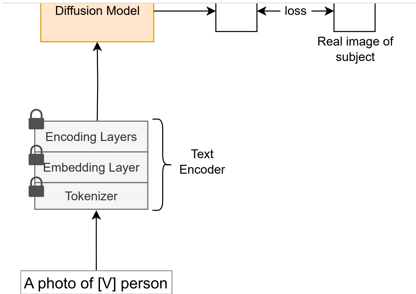
Figure 7: DreamBooth method updating the entire diffusion model
