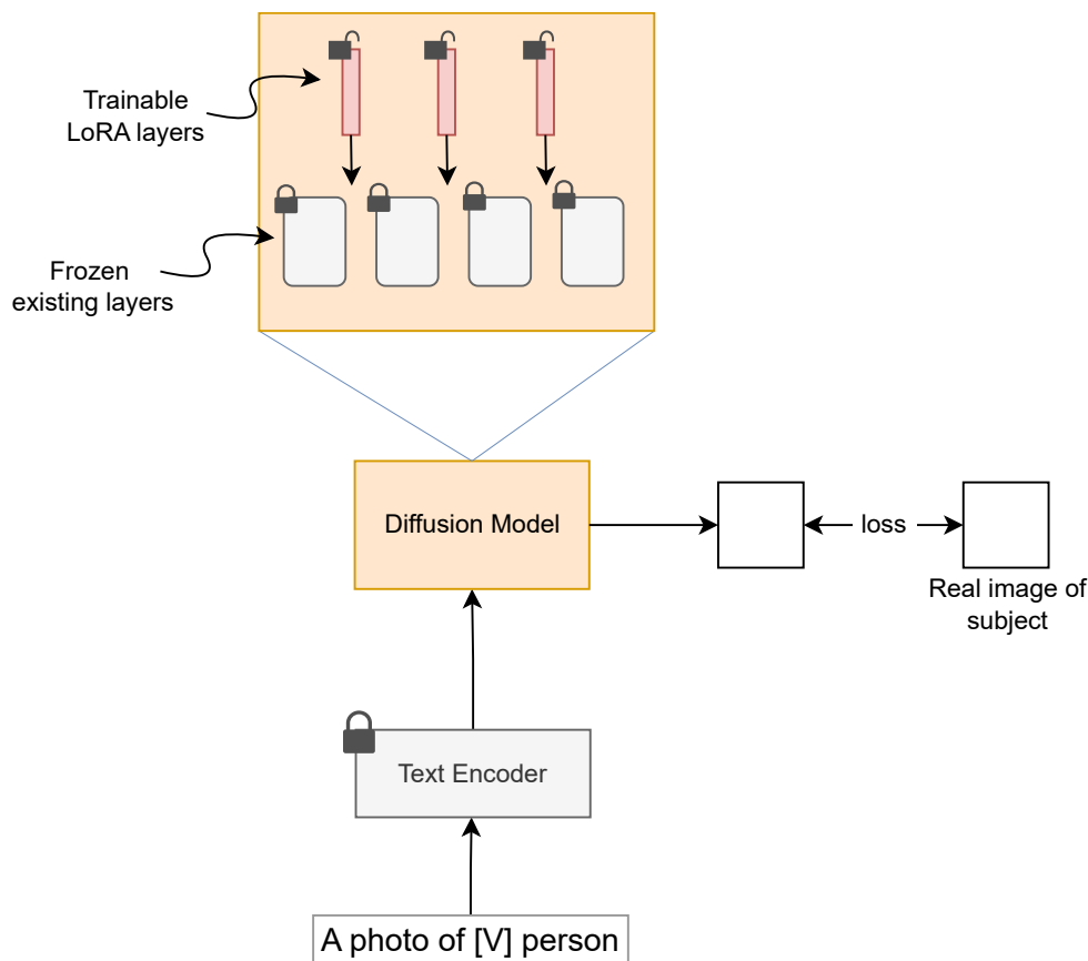
Figure 10: LoRA method injecting and learning new parameters in the diffusion model
