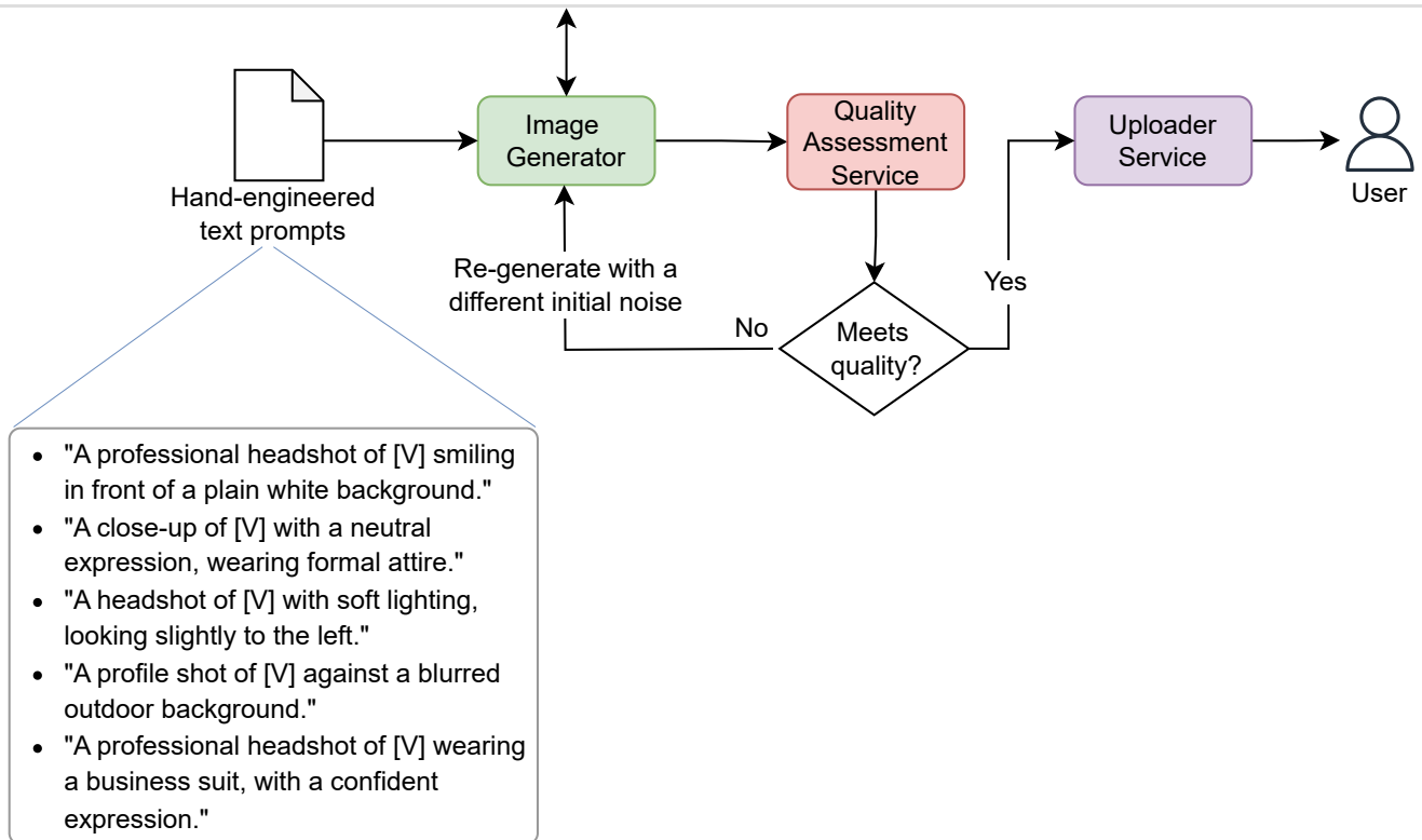
Figure 18: Inference pipeline components
